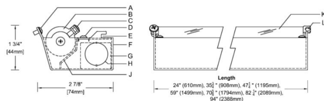
Cove Design 1:4 Scale
