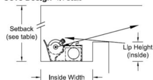
Cove Design 1:4 Scale
